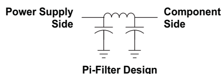
Figure 2. Filter Designs
