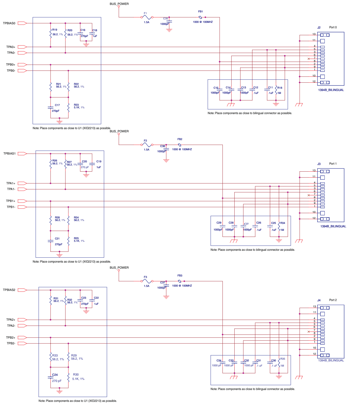
Figure 5. 1394b Connector
